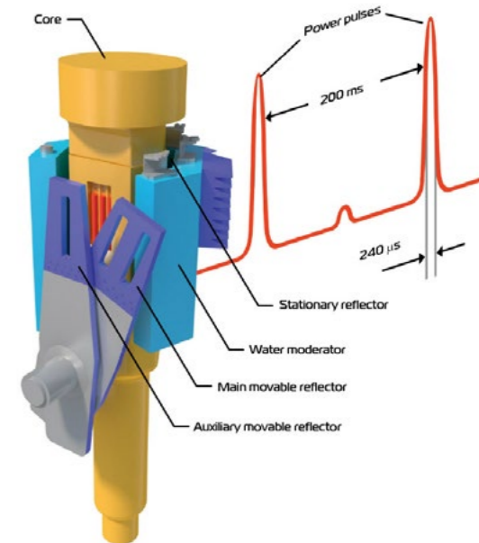
Schematic representation of the IBR-2 Reactor's operation
